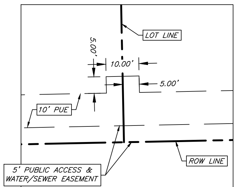
Typical 5'x10' Easement Extension N.T.S.
